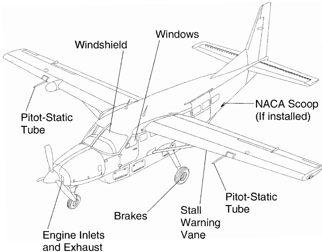
Figure 4 C208 Sensitive Areas
