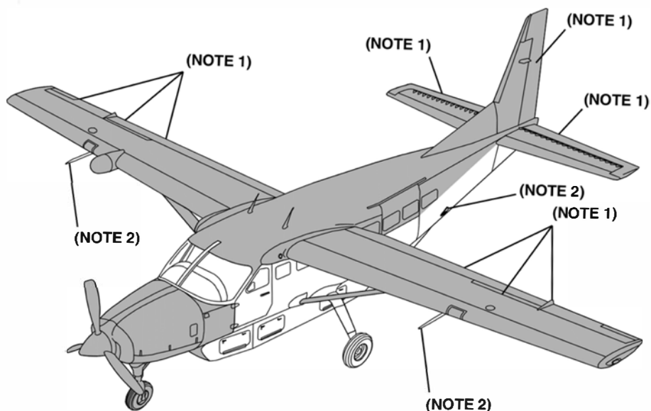
Figure 2. C208 critical deice and inspection areas
