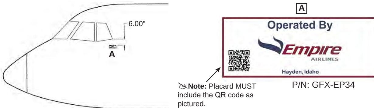
Figure 1 - LH shown, RH installed in same location
